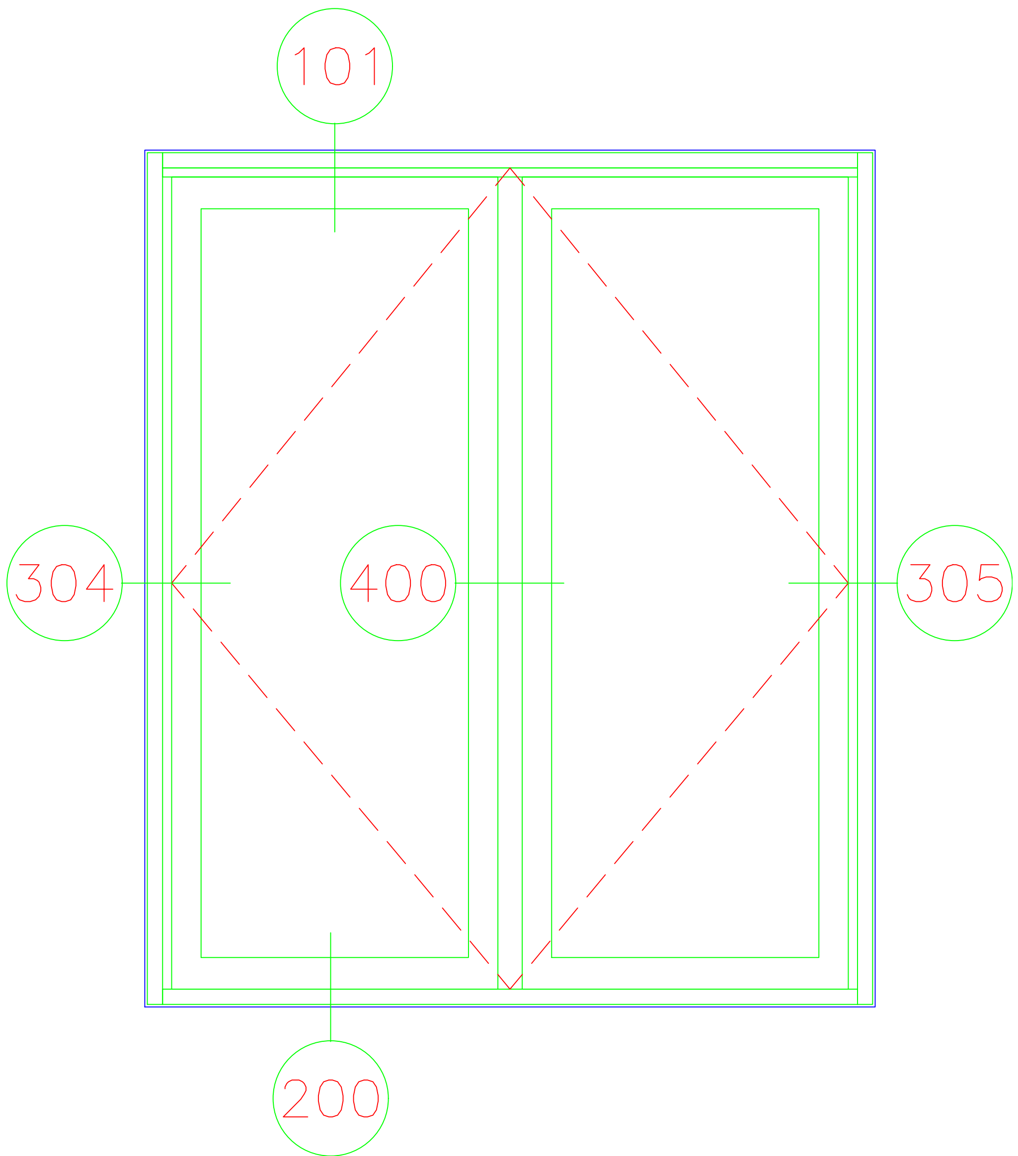
T325i Outswing Standard Frame Door Pair Left and Right Swing Butt Hinges Multipoint Rolling Cam Locks
